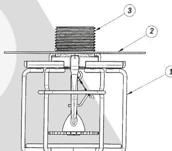
1 - Guard, Model 25 2 - Shield, ESFR 3 - Sprinkler Assy, Model N25 ESFR
