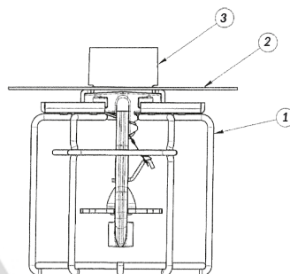
1 - Guard, Model 22 2 - Shield, ESFR 3 - Sprinkler Assy, Model HL22
