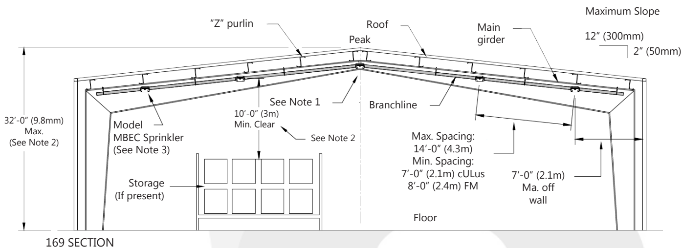
Figure 2. Installation Detail A.
