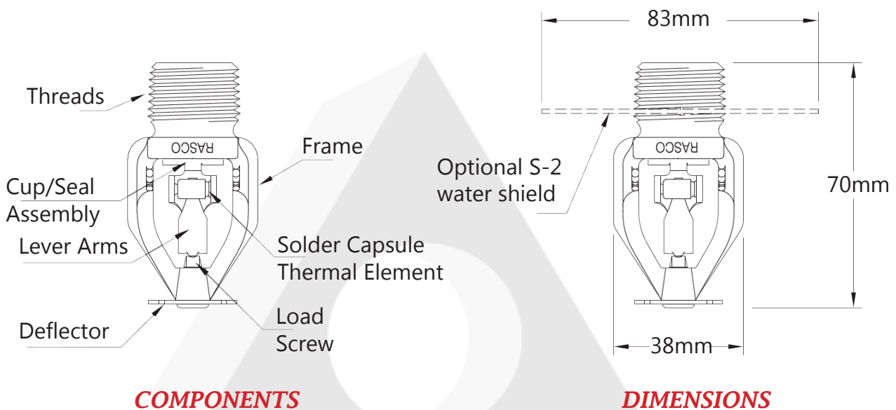
Fig. 2 - Model GXLO Pendent Components and Dimensions
