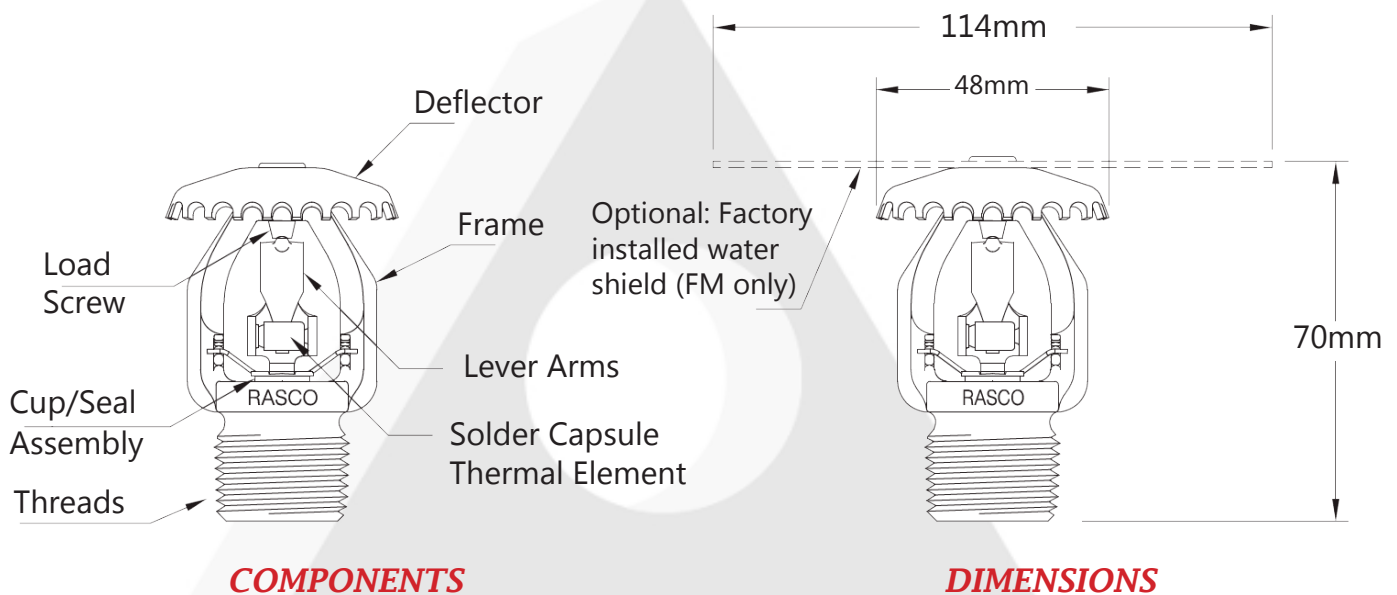
Fig. 1 - Model GXLO Upright Components and Dimensions
