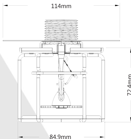
Model 25 Guard w/ S-5 Shield
