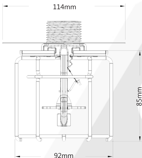
Model 22 Guard w/ S-5 Shield
