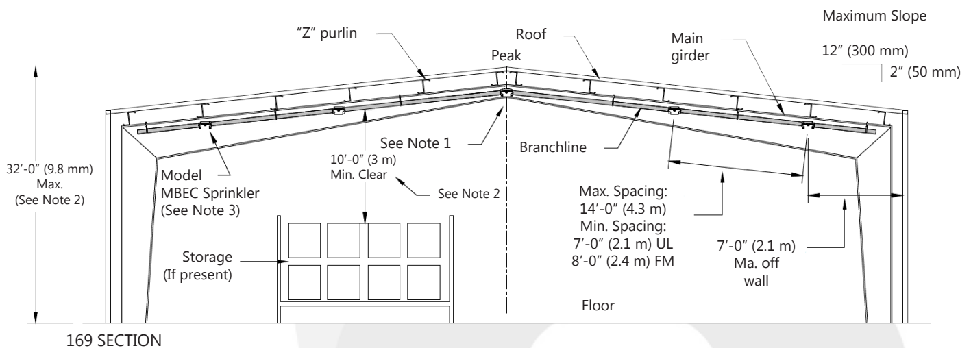
Figure 2. Installation Detail A.
