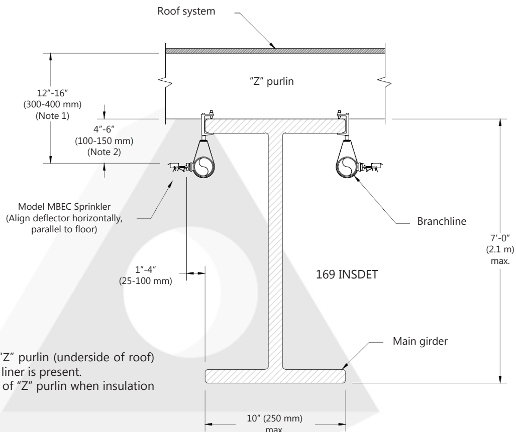
Figure 3. Installation Detail B.
